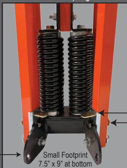
Heavy Duty Double Spring
