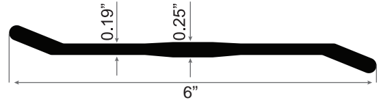
Rail Dimensions
